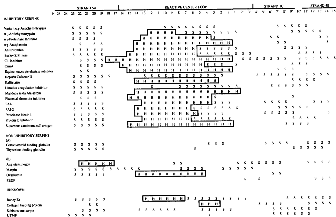
Fig. 2. Secondary structure predictions (winner-takes-all) for all serpins examined. The letters S and H signify prediction for \beta -strand and \alpha -helix respectively. Blank spaces signify no prediction for \beta -strand or \alpha -helix. The sequences used and the alignments for determining the position of the P1–P1' residues were from the literature.
